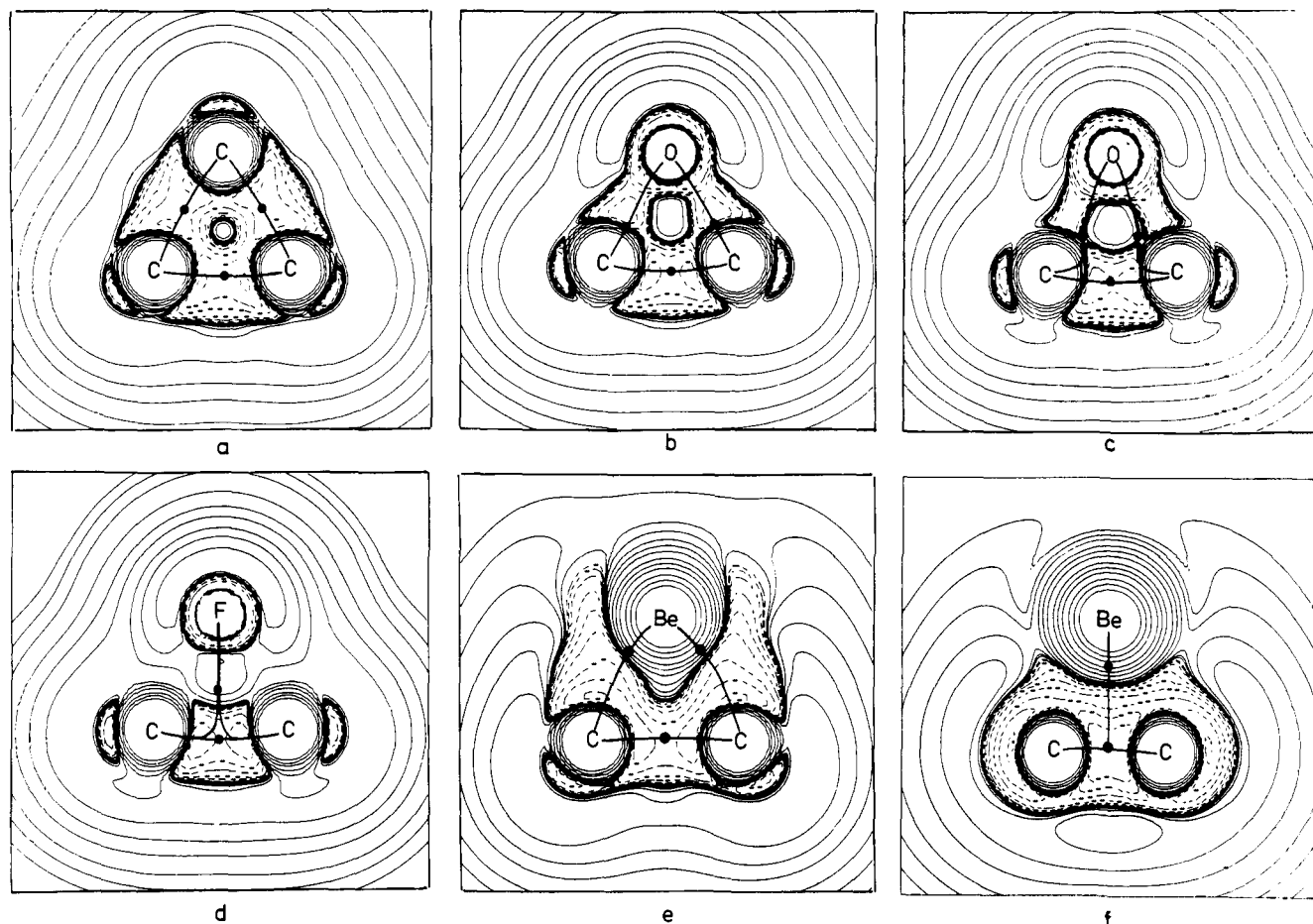
Figure 1. Molecular graphs and Laplace concentrations, \nabla^2\rho(r) , of cyclopropane (a), oxirane (b), protonated oxirane (c), halogen-bridged fluoroethyl cation (d), berylliocyclopropane (e), and berylliocyclopropine (f). Bond paths are indicated by heavy lines and bond critical points by dots. Dashed lines are in regions where electronic charge is concentrated ( \nabla^2\rho(r) < 0 ) and solid lines in regions where charge is depleted ( \nabla^2\rho(r) > 0 ). HF/C//C calculations.
