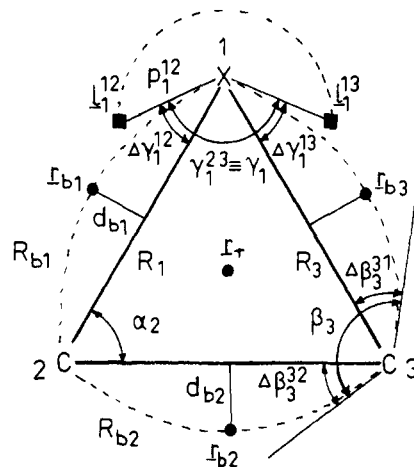
Figure 4. Geometrical parameters used for the description of critical points of \rho(r) ( r_b, r_\tau ) and -\nabla^2\rho(r) ( l^j ). Compare with Table III. Bond paths are indicated by dashed lines. The semicircle around 1 symbolizes part of the valence sphere of 1.
